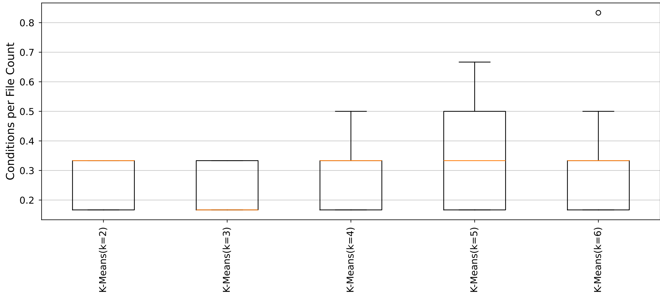
YARA Rules Conditions per File Count Distribution (Cluster27_Size6 dataset)
